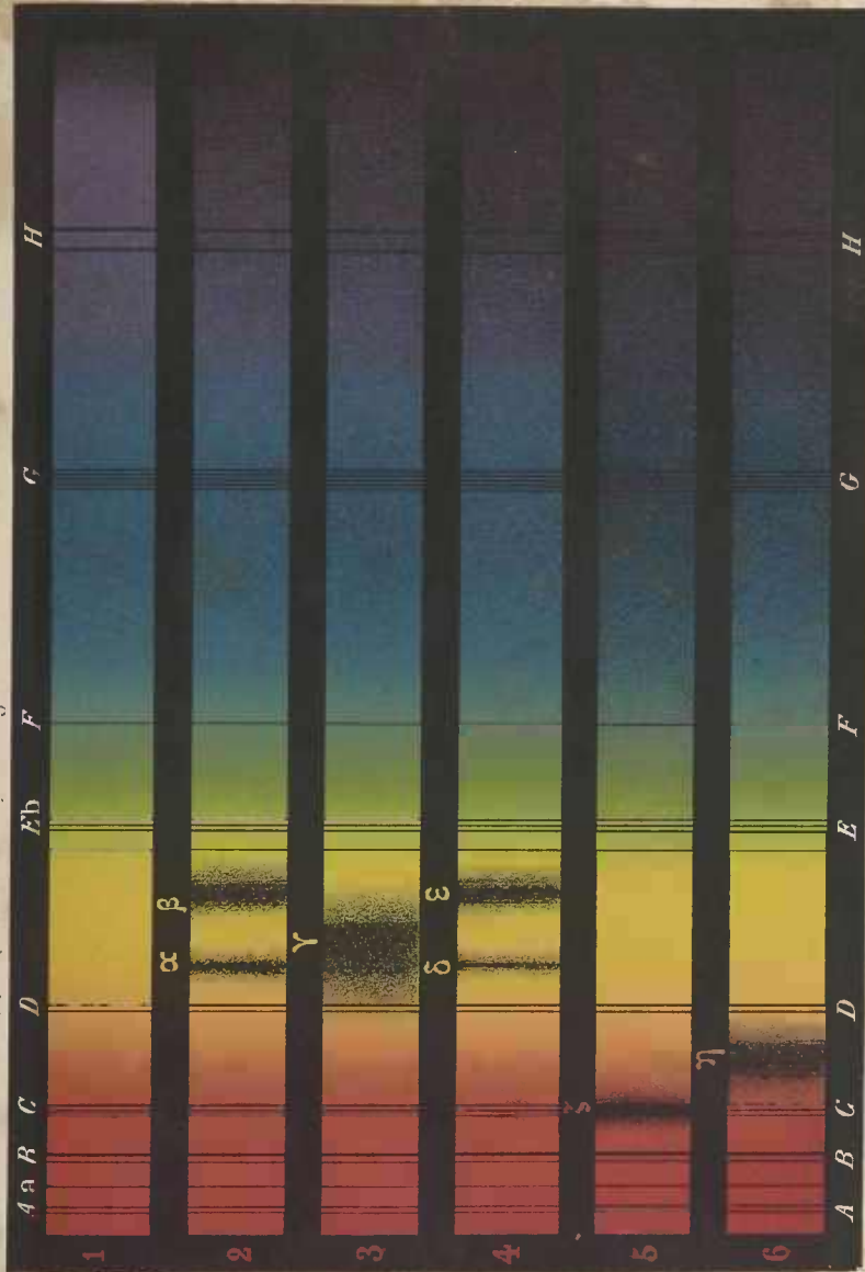
1 Spectre solaire
